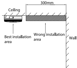
Figure 4-3 Installation position (2)
