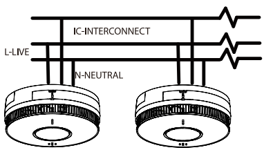
Figure 5-1 Interconnection
