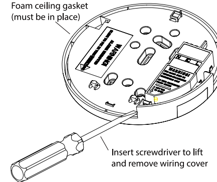
Figure 4-6 Installation (2)
