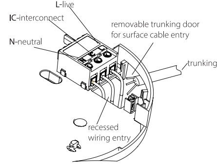
Figure 4-8 Installation (4)
