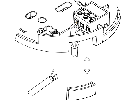
Figure 4-8 Installation (4)
