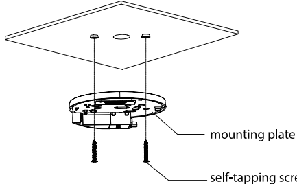
Figure 4-5 Installation (1)
