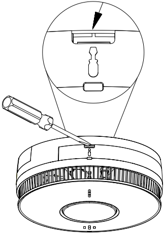
Figure 4-10 Removal
